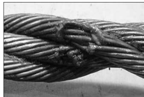
a. Heat damage from welding.
